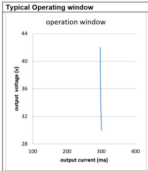
Operating Window
